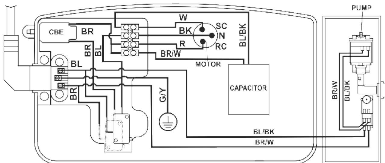
Electrical Layout For P Model
